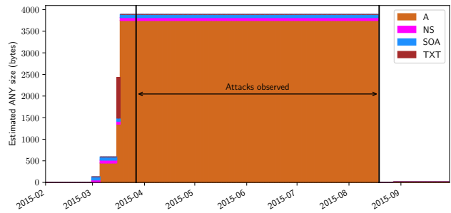
Figure 2: Example of an artificially inflated domain ( sunrisecx.com )
