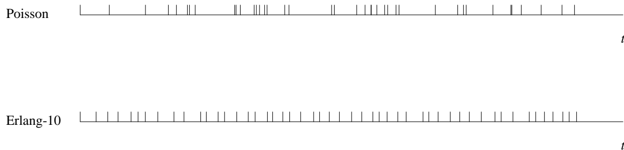
Figure 2.6: A realization of Poisson arrivals and Erlang-10 arrivals, both with rate 1
