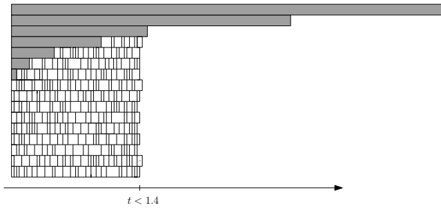
Figure 2: Schedule with value v^* : all long jobs start at time 0, yet some of these machines are expected to become available for processing short jobs.
